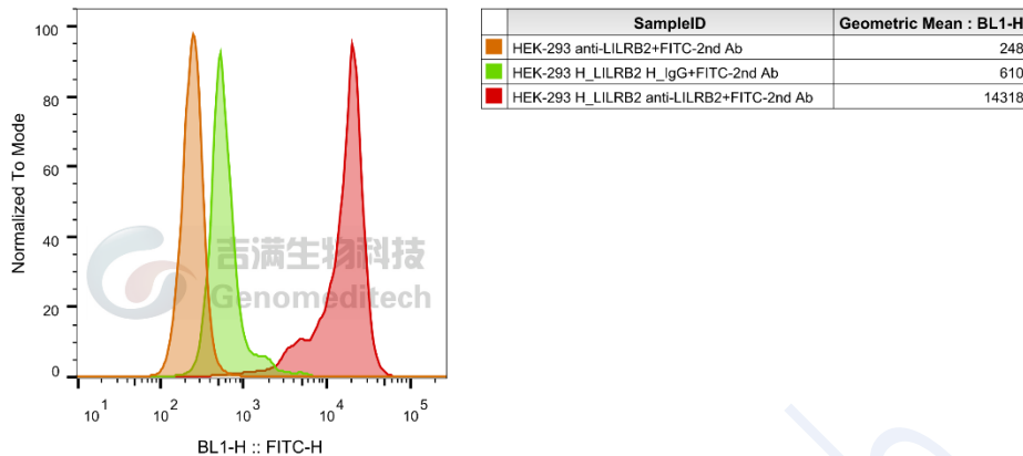
Figure 1 | H_LILRB2(ILT4) HEK-293 Cell Line was determined by flow cytometry using Anti-H_LILRB2(ILT4) hIgG4 Antibody(MK-4830) (Genomeditech/GM-27362AB).
